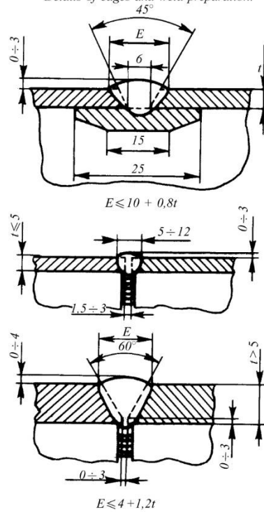
Fig. 5 Test piece of pipe joint with a limited access to the welding zone P 5
