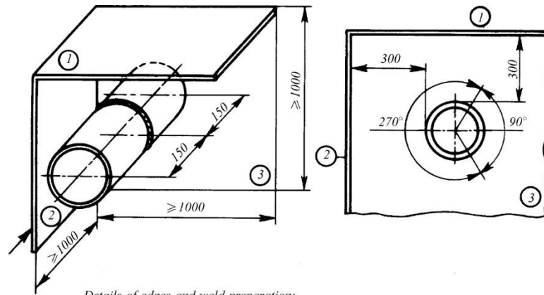
Fig. 4 Test piece of P 4 fillet-welded pipe joint
